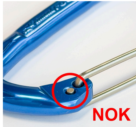
Photo 2: NOK riveting, flat end
