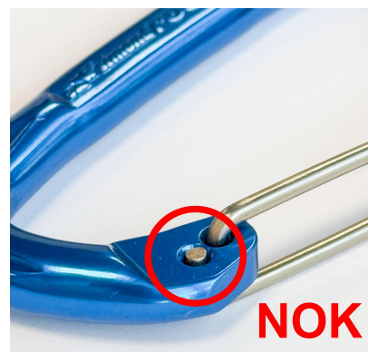
NOK riveting, flat end
